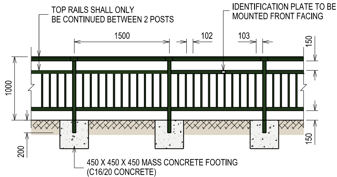
TYPE B ALUMINIUM ALLOY RAILINGS
