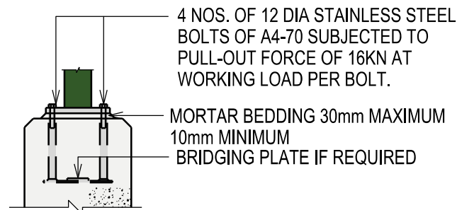
TYPICAL DETAIL OF RAILING FIXING TO CONCRETE STRUCTURE BY CAST-IN CRADLES
